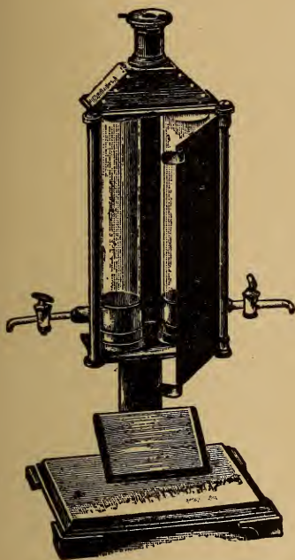
Fig. 94. WOLFF'S COLORIMETER, FOR INSPECTING ANILINE DYES.
